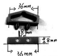
36mm EURO BLACK PLASTIC TAB
